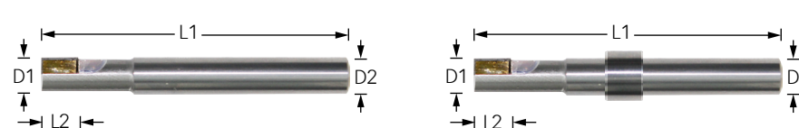
PXXX-A with stop ring (A-Version)
